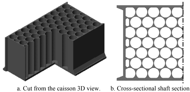
Figure 1. Generic views of a typical floating caisson
