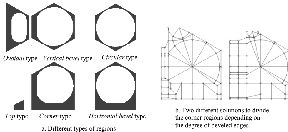
Figure 3. Basic regions that define the cross-sectional shaft section
