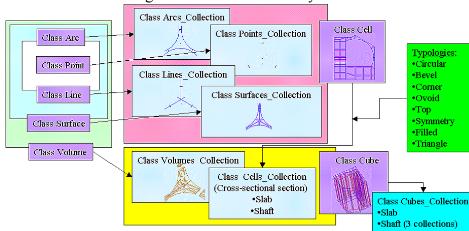
Figure 6. Scheme of classes used in the algorithm
